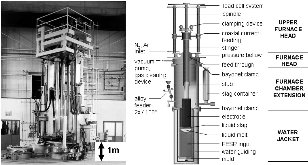
Figure 11: Appearance and configuration of modern P-ESR-plant
