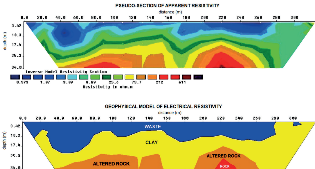
Figure 8. Pseudo-section of electrical resistivity from landfill
